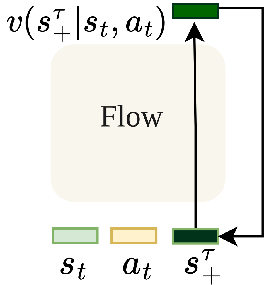
a) Geometric Horizon Model Learning
